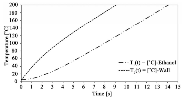
Figure 5. Time-history of temperature rise of ethanol and the inner injector wall in function of the time to a heating power of 100 W e \bar{h} = 300 \text{ W/m}^2\cdot^\circ\text{C} .
